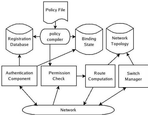
High-level view of Controller components.
