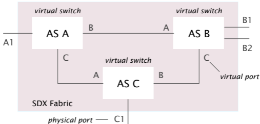
(a) Virtual switch abstraction.
