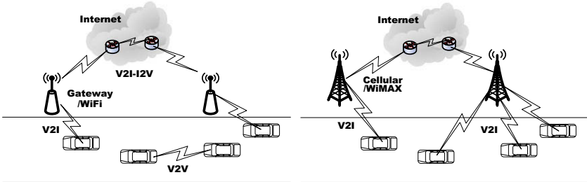
(b) Cellular/WiMax
